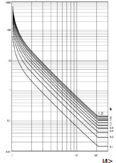
Extremely Inverse (EI 0.65)*
