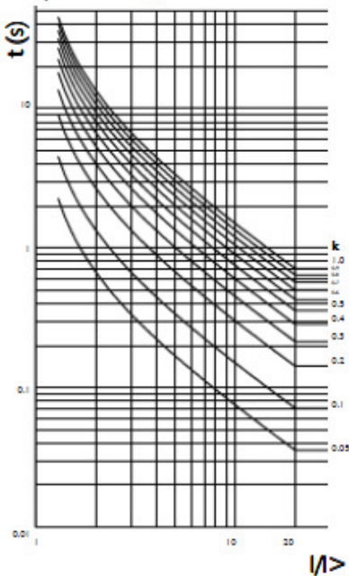
Very Inverse (VI)*
